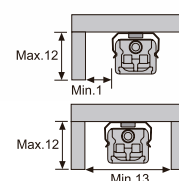
Standard mounting
