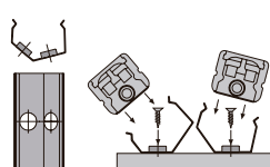
NDV-BRACKET2
